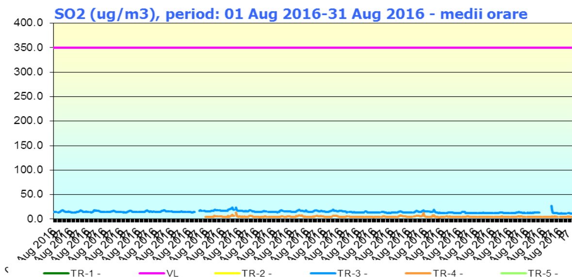
Fig. 1.1 - SO 2 (μg/m 3 ), August 2016
