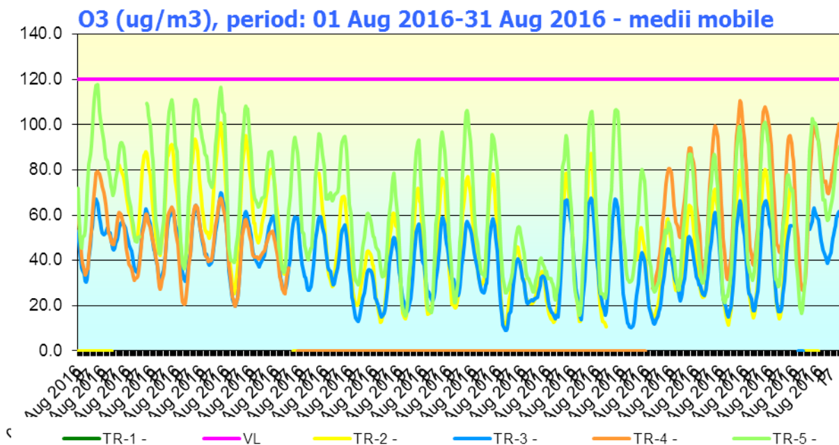
Fig. 1.3 - O 3 (μg/m 3 ), August 2016
