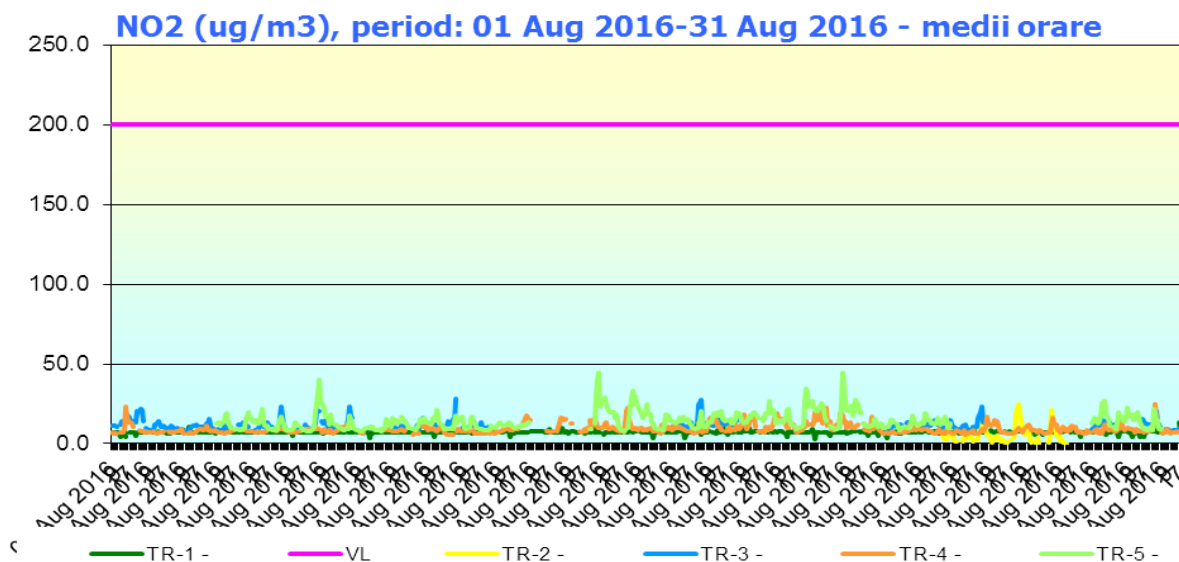
Fig. 1.2 - NO 2 (μg/m 3 ), August 2016
