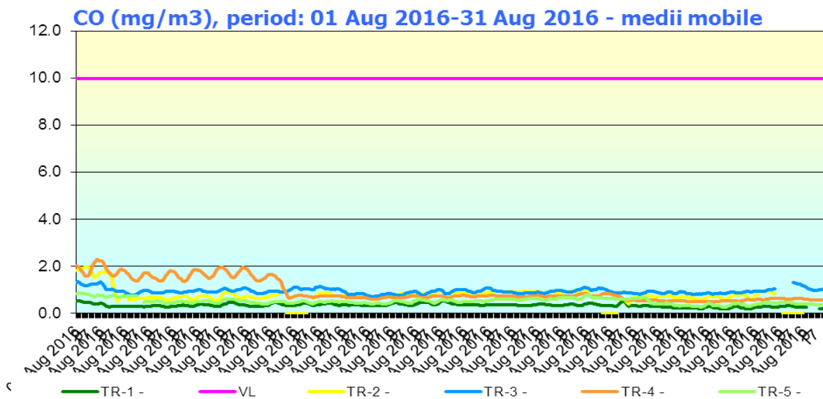
Fig. 1.4 - CO (mg/m 3 ), August 2016
